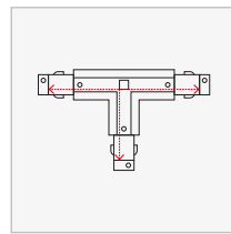
T Joiner 3 Way (TR2) TRA3C-TR2 White | Black | Silver Power feeding possible
