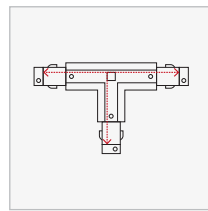
T Joiner 3 Way (TR1) TRA3C-TR1 White | Black | Silver Power feeding possible
