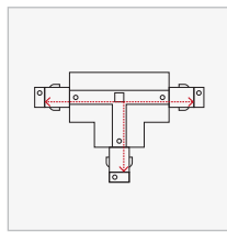
T Joiner 3 Way (TL2) TRA3CR-TL2 White | Black | Silver Power feeding possible
