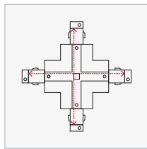
X Joiner 4 Way (XJ) TRA3CR-XJ White | Black | Silver Power feeding possible
